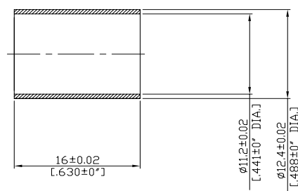
RG-214 Ferrule
