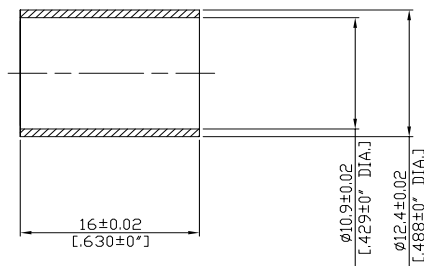
RG-213 Ferrule
